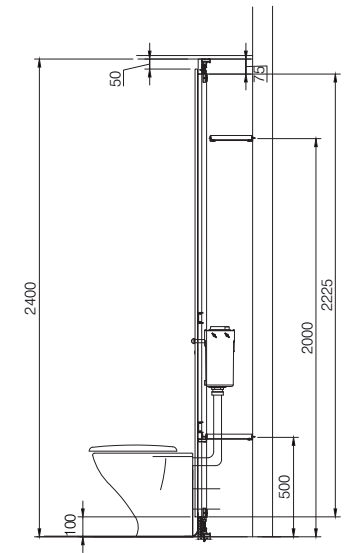
Section Detail
